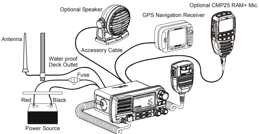
Figure 1. General Installation
